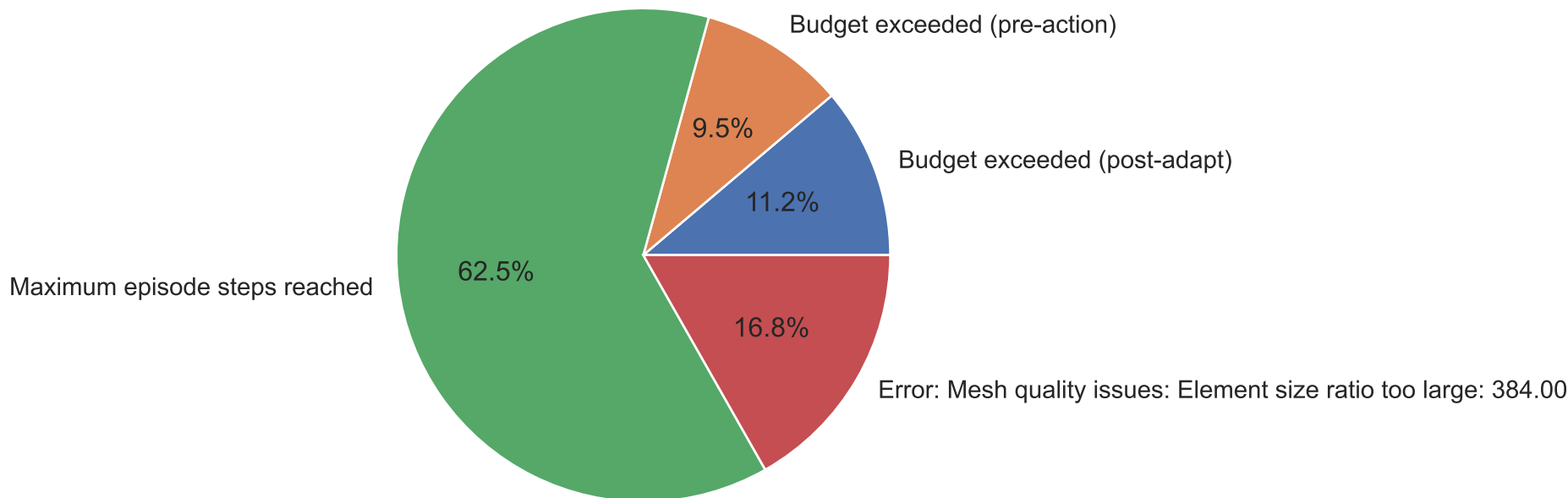
Episode Termination Reasons
