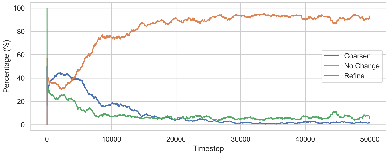
Action Distribution Evolution
